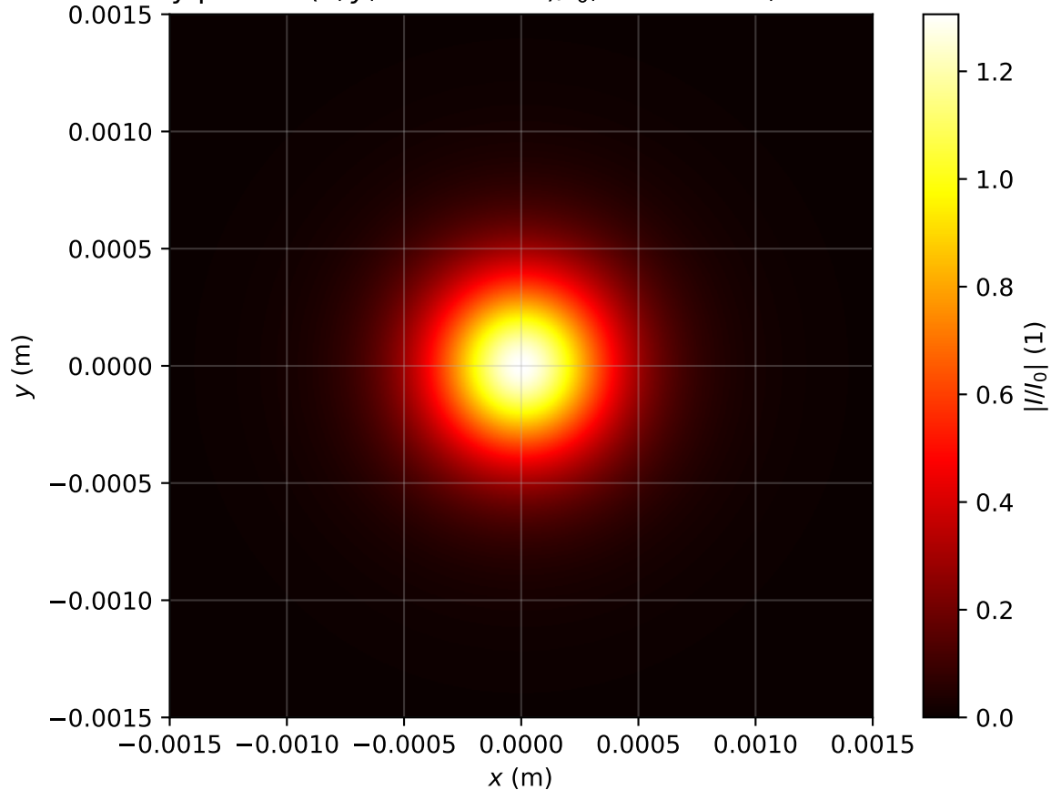
Intensity profile I(x, y, z = 2.070m)/I_0 , P_{in}=0.8P_{cr} , artificial time
